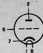
Loctal B8G
